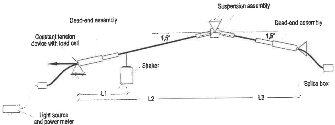
Figure 1: Schematical diagram of test set-up (L1 = 8,54 m, L2 = 28,14 m, L3 = 12,45 m)
