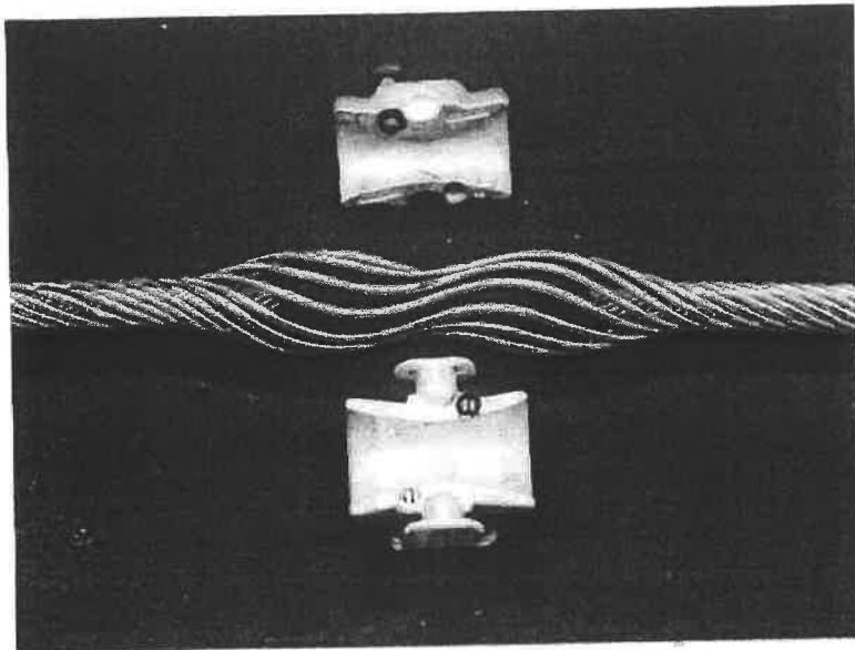
Figure 10: After test, clamp housing taken off, no damage.
