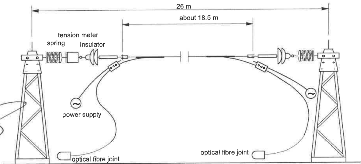
Figure 1: Test arrangement.
