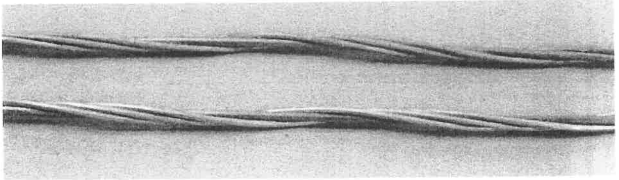
Fig. 2: Four wires of outer wire layer unwrapped. View of stainless steel tube. Bottom cable specimen, no exposure to salt spray. Top cable specimen after test.
