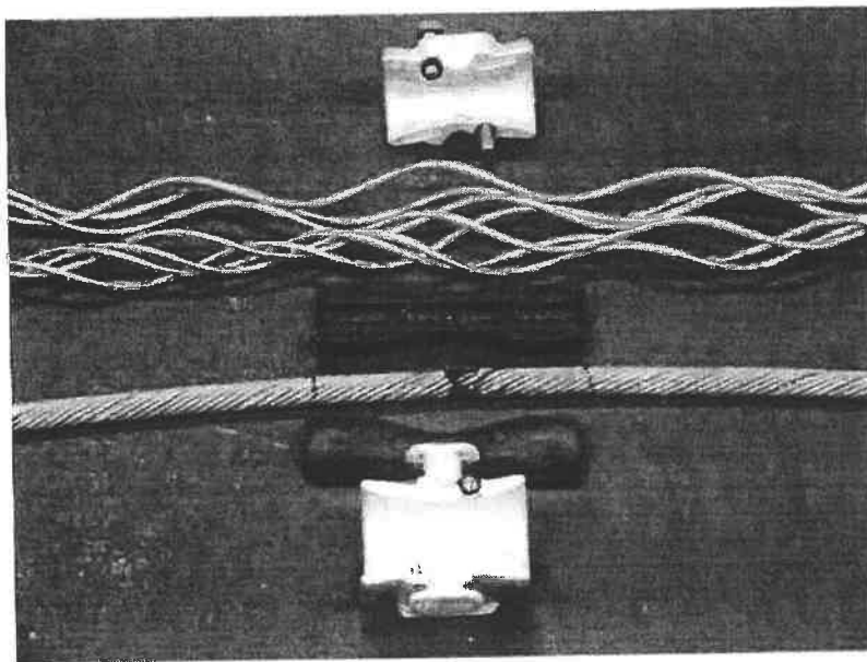
Figure 11: After test, view on protection rods on cable, armour rods and neoprene inserts taken off, no damage.
